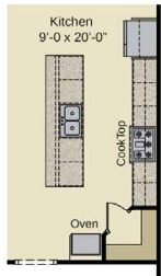
Gourmet Kitchen 1/4" = 1'-0" (OPTIONAL)
